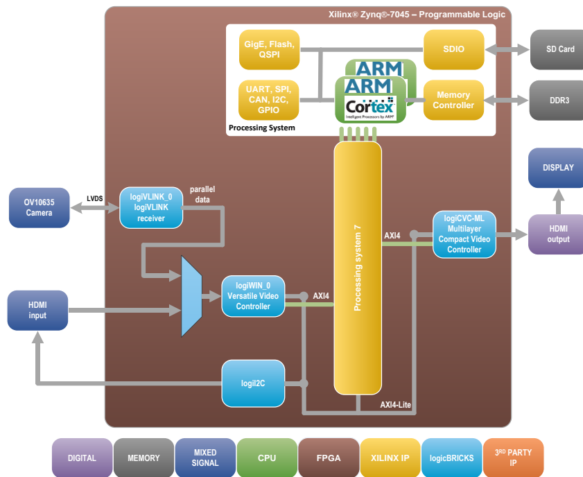
Figure 12: CAM-HDMI SoC Design – Block Diagram (Pre-Defined Platform)
