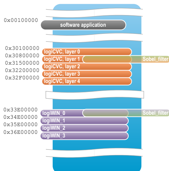
Figure 17: FOUR-CAM Design Memory Layout
