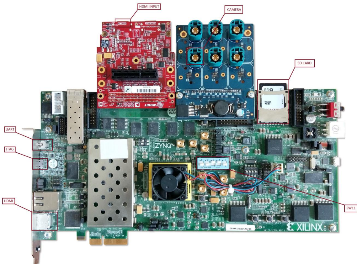
Figure 20: CAM-HDMI HW Setup
