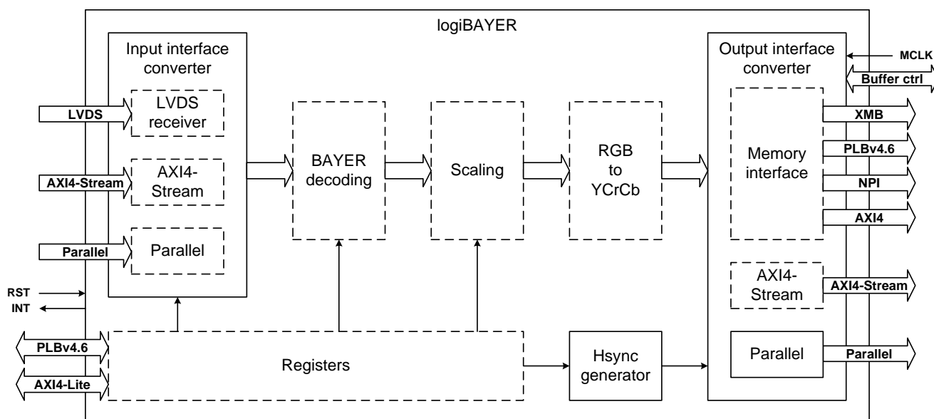
Figure 1: logiBAYER Architecture
