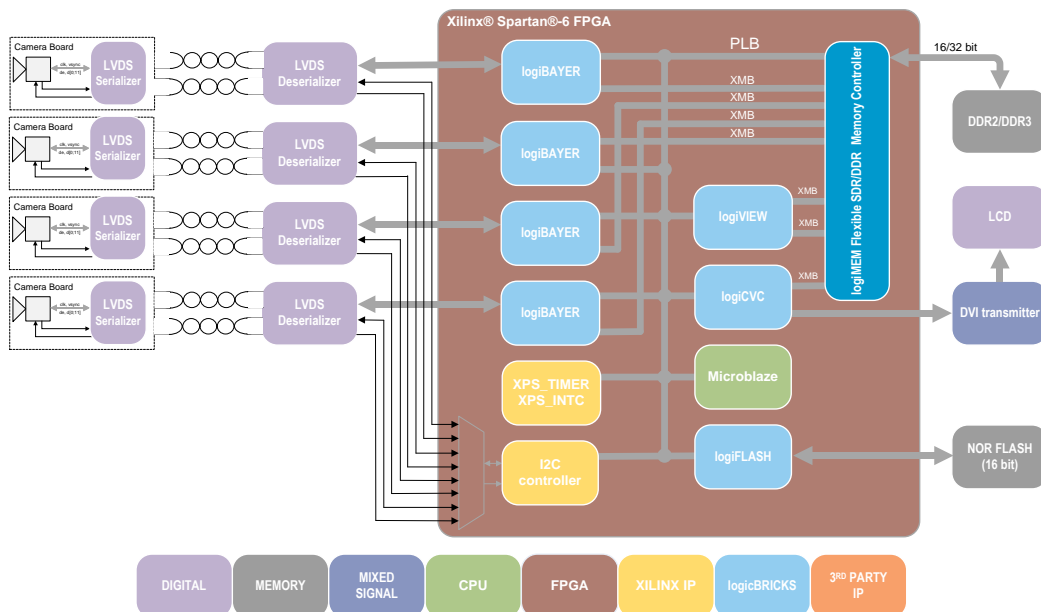
Figure 3: An Example FPGA Architecture – 4x logiBAYER in Automotive Surround View System
